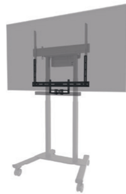
AV2-500BL Screen size: 43-110" Capacity: 10 kg VESA: 200x200 - 800x600
